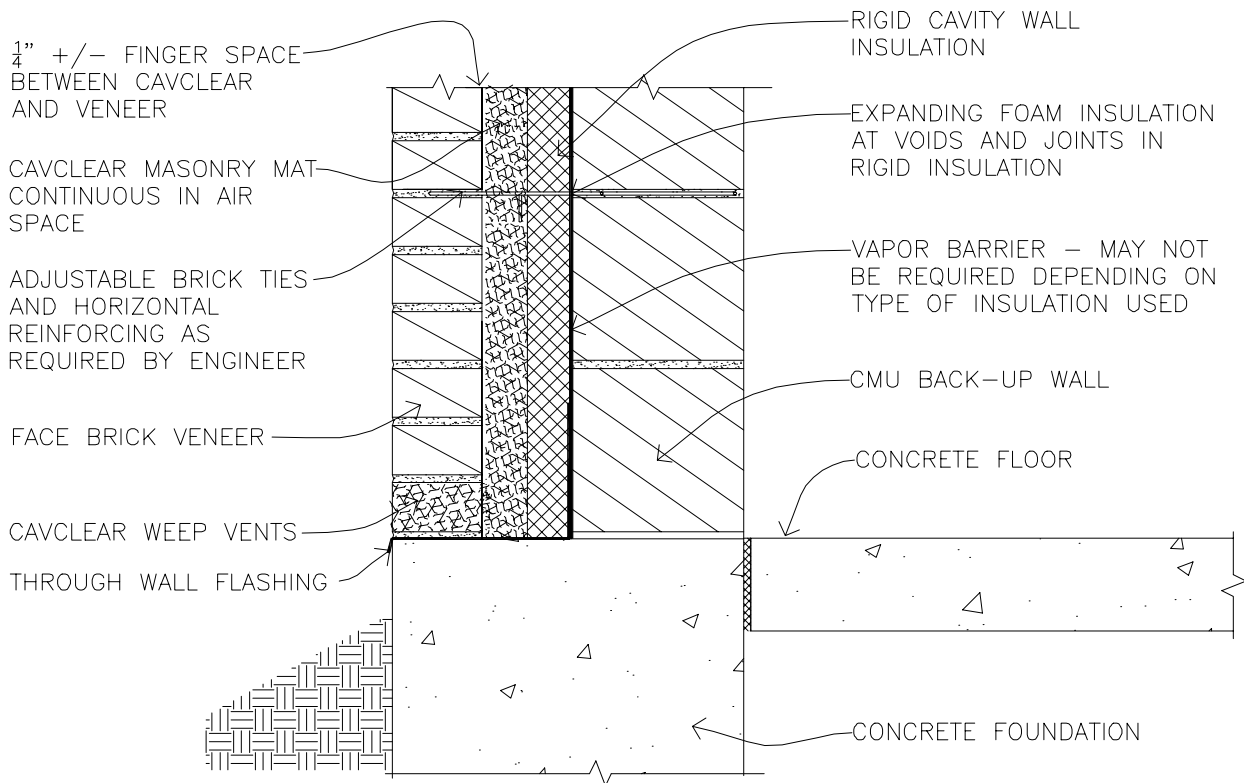
BRICK VENEER CAVITY WALL WITH CMU BACKUP
