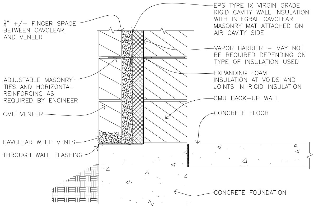
CMU VENEER CAVITY WALL WITH CMU BACKUP AND CAVCLEAR EPS INSULATION SYSTEM
