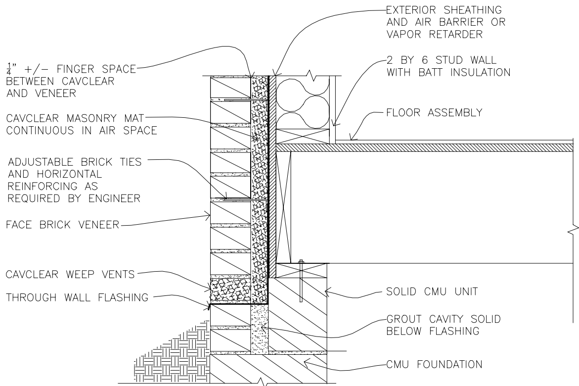
TYPICAL RESIDENTIAL BRICK VENEER CAVITY WALL WITH STUD WALL BACK-UP
