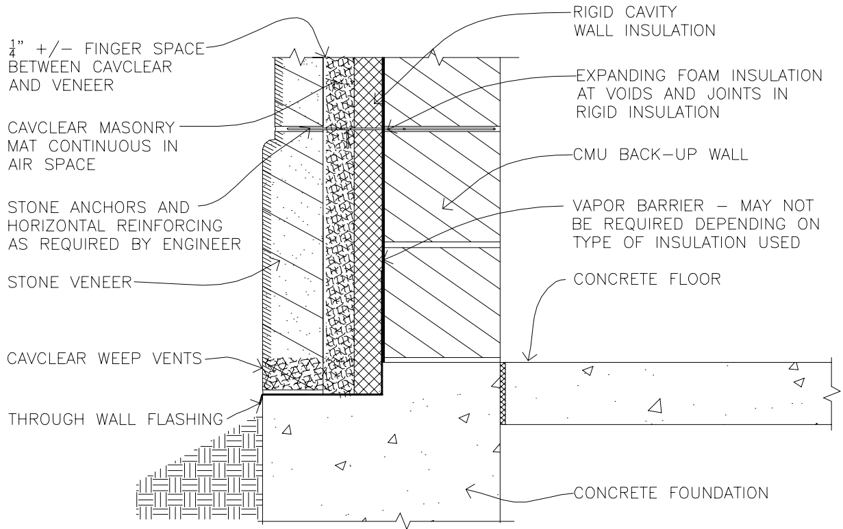
STONE VENEER CAVITY WALL WITH CMU BACKUP
