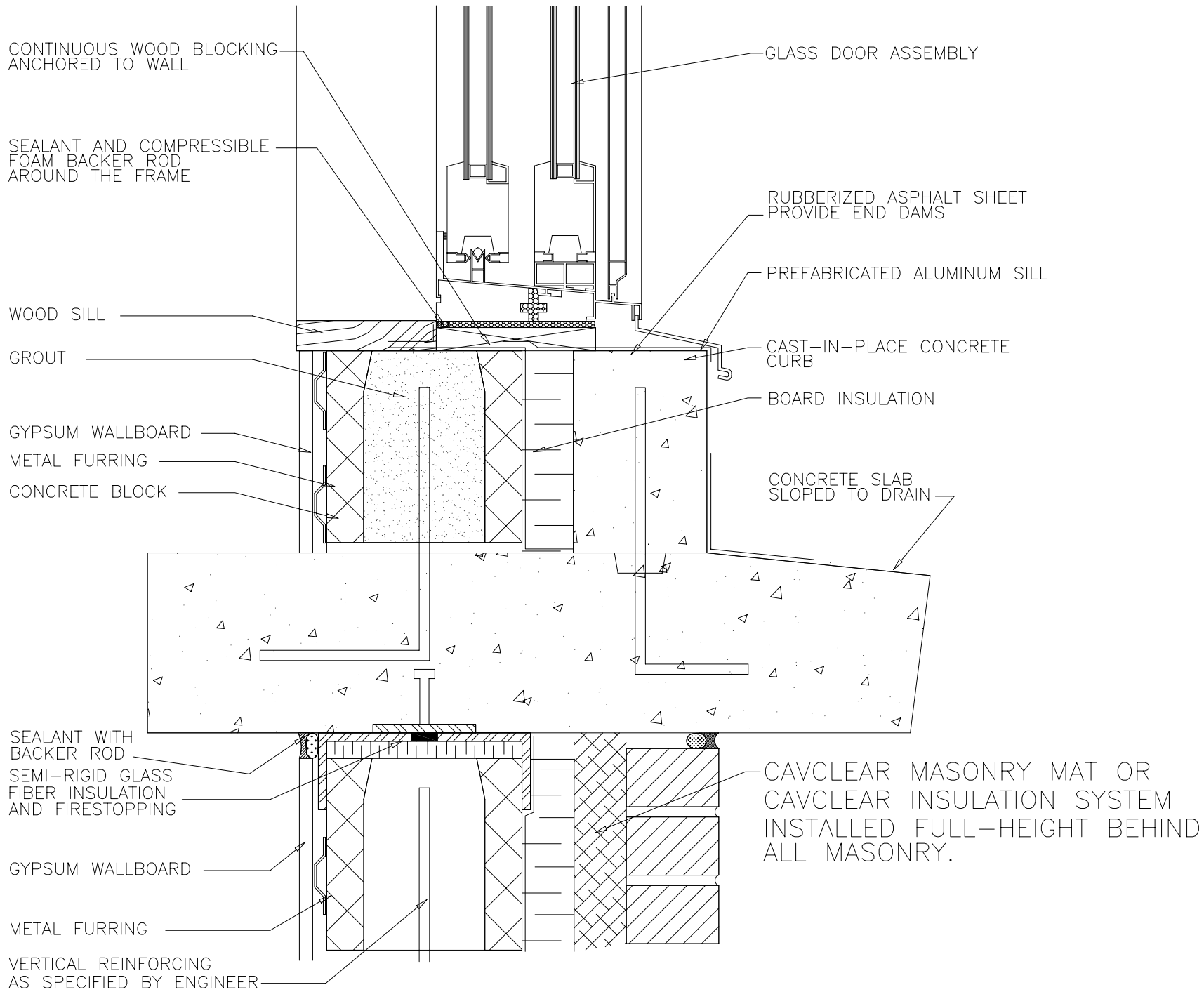
BALCONY FLOOR AT DOOR DETAIL
