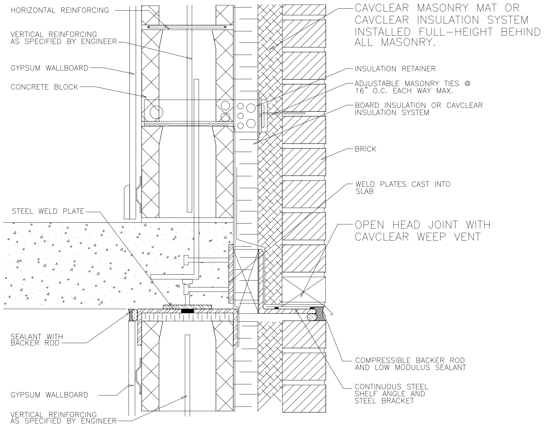
BRICK SHELF ANGLE DETAIL
