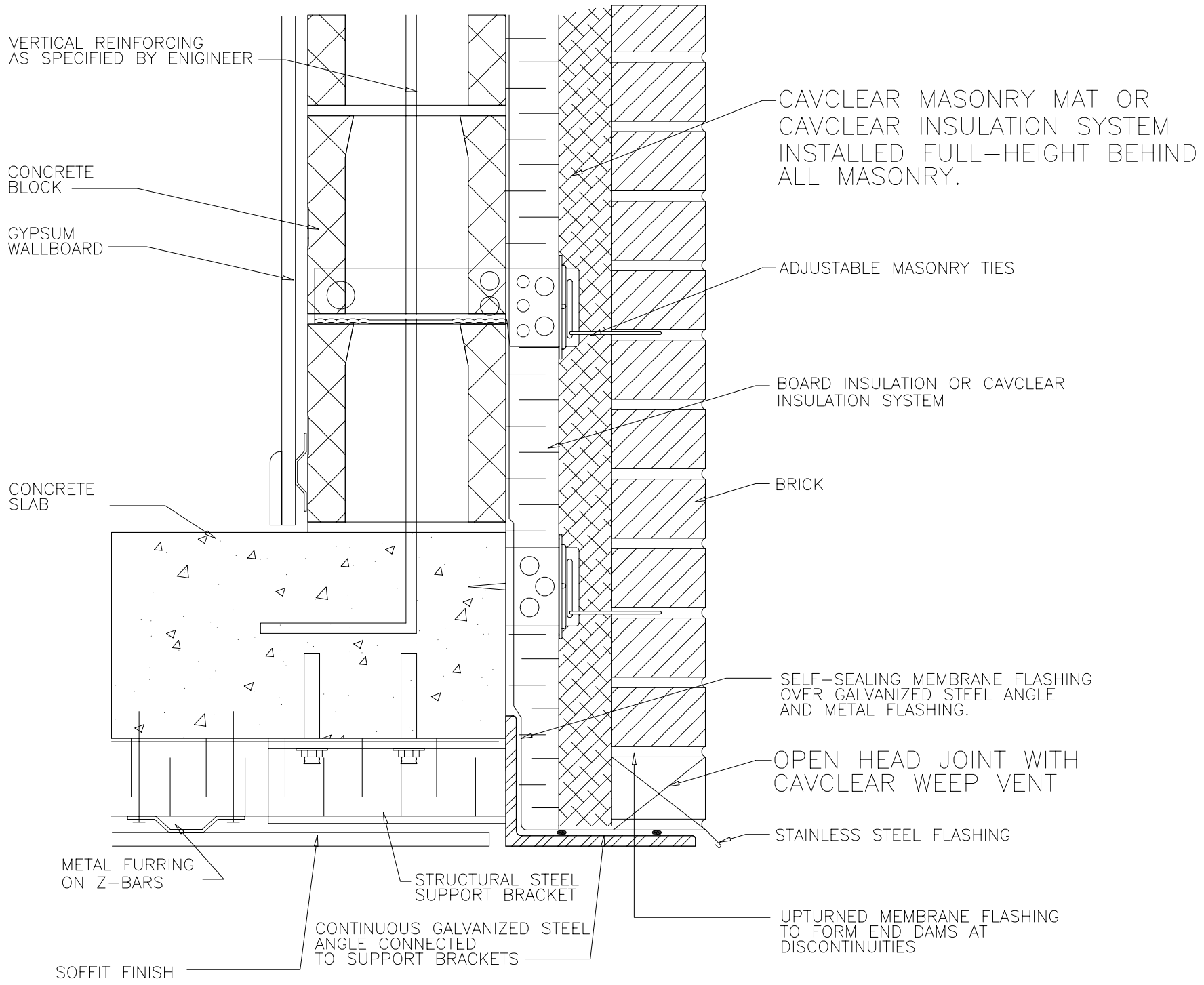
CONTILEVERED SOFFITT AND SHELF ANGLE DETAIL
