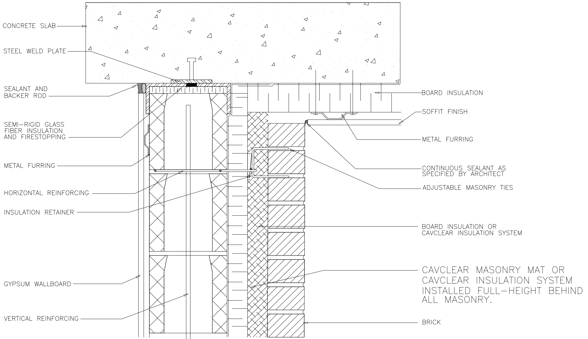
CANTILEVERED SOFFIT AT WALL DETAIL
