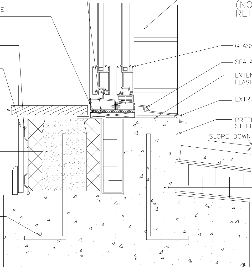
DOOR ABOVE LOW SLOPE ROOF DETAIL
