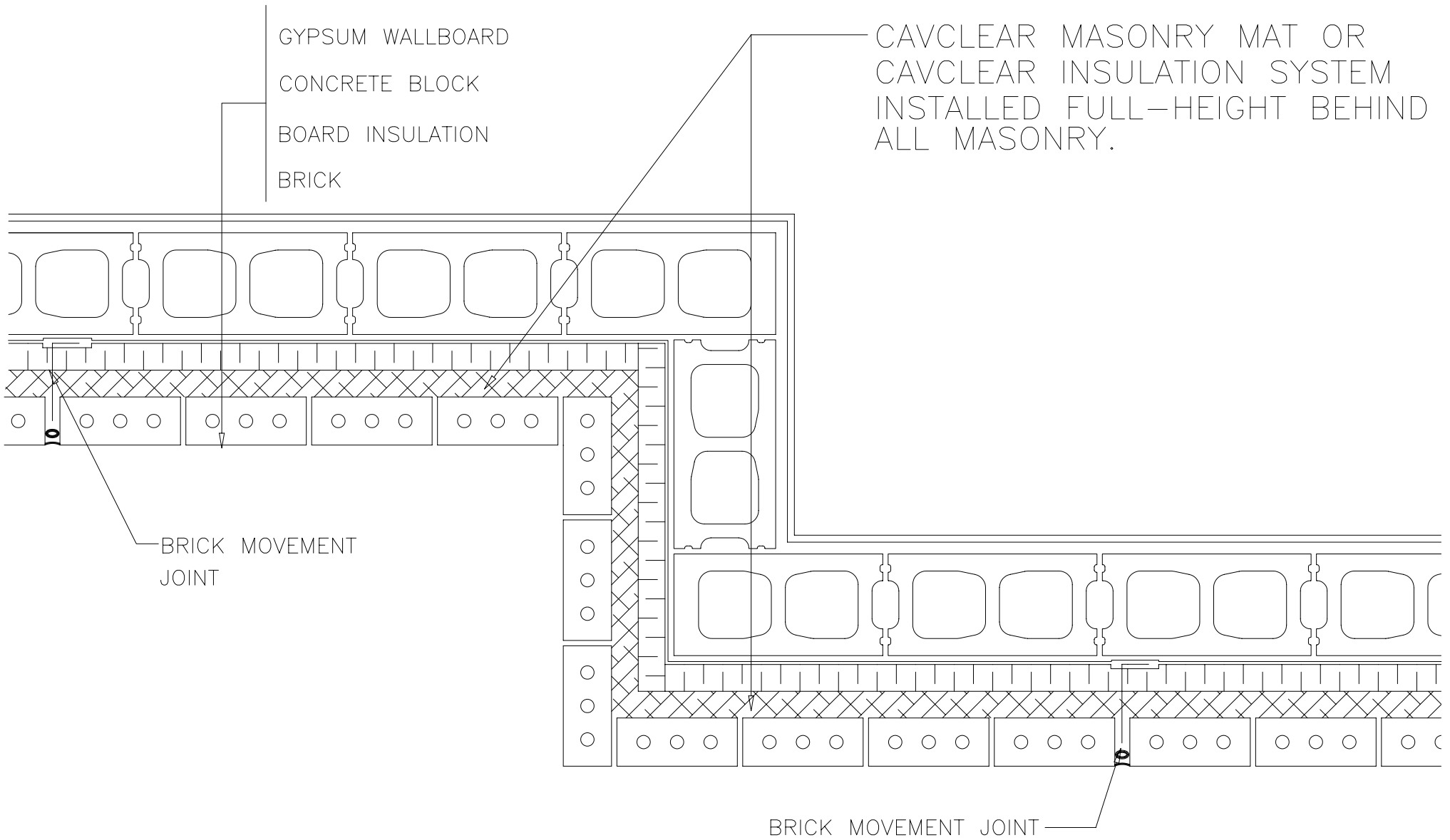
EXTERIOR AND INTERIOR CORNERS DETAIL
