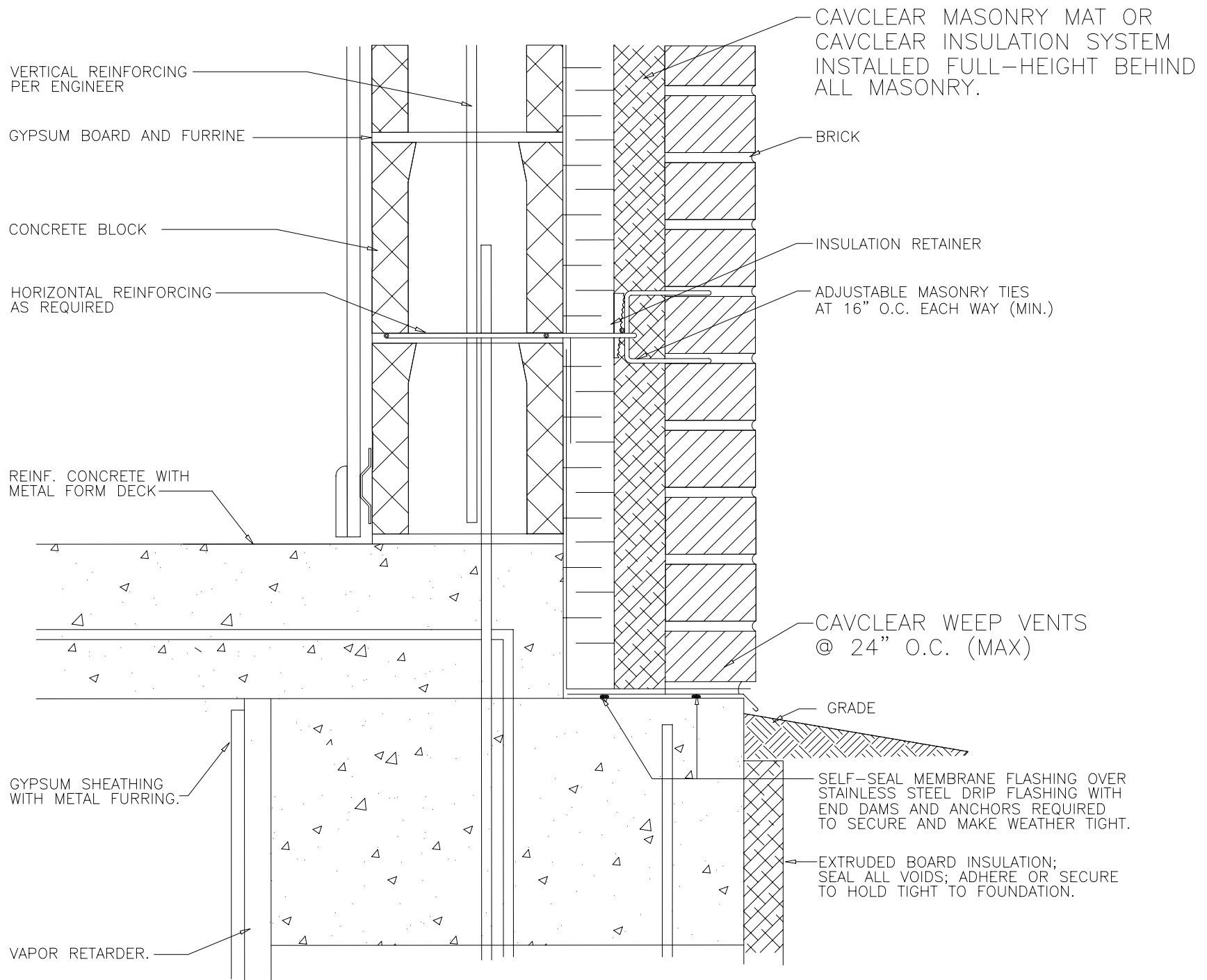
FOUNDATION OR BRICK LEDGE DETAIL
