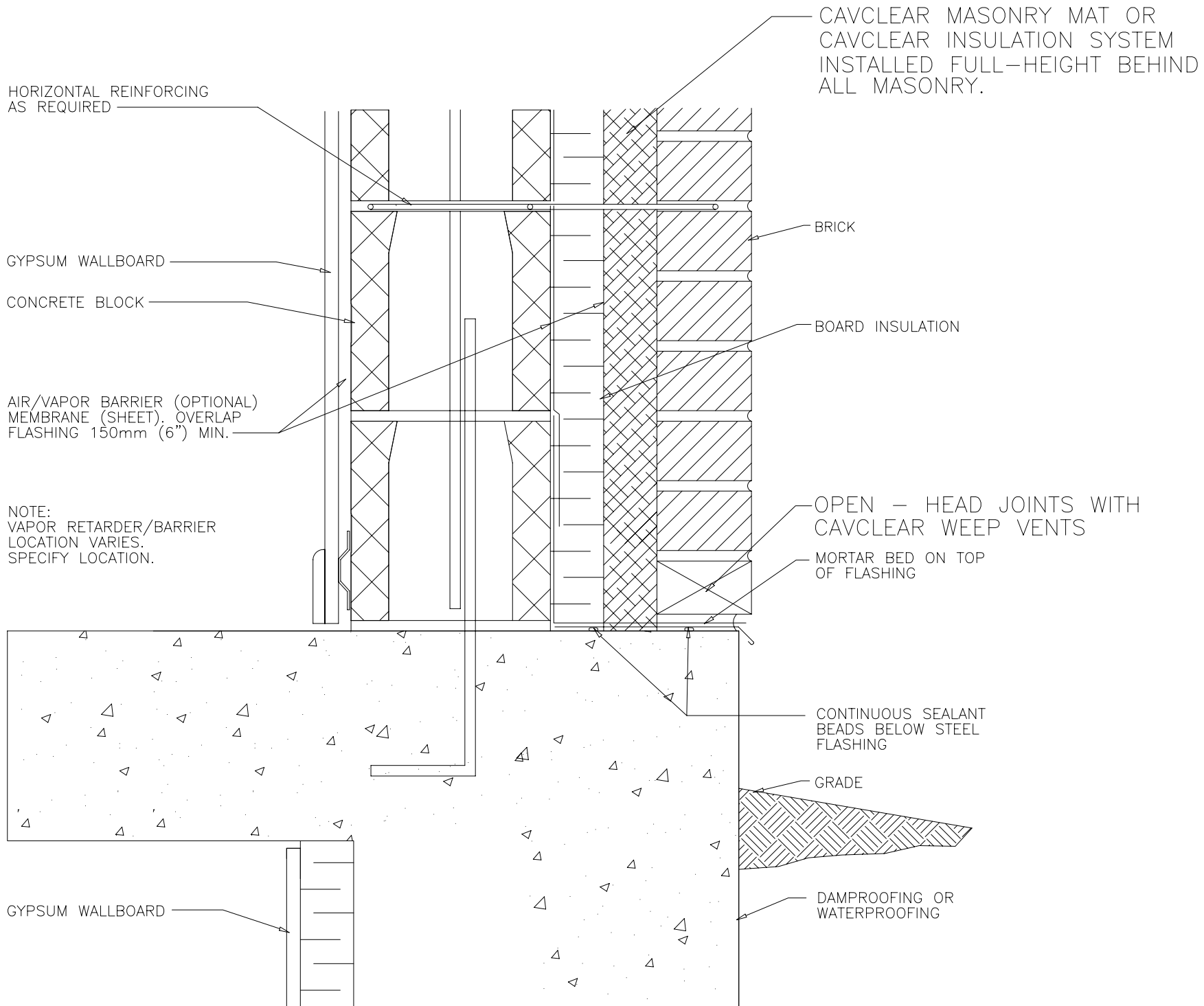
FOUNDATION WITH BRICK LEDGE DETAIL
