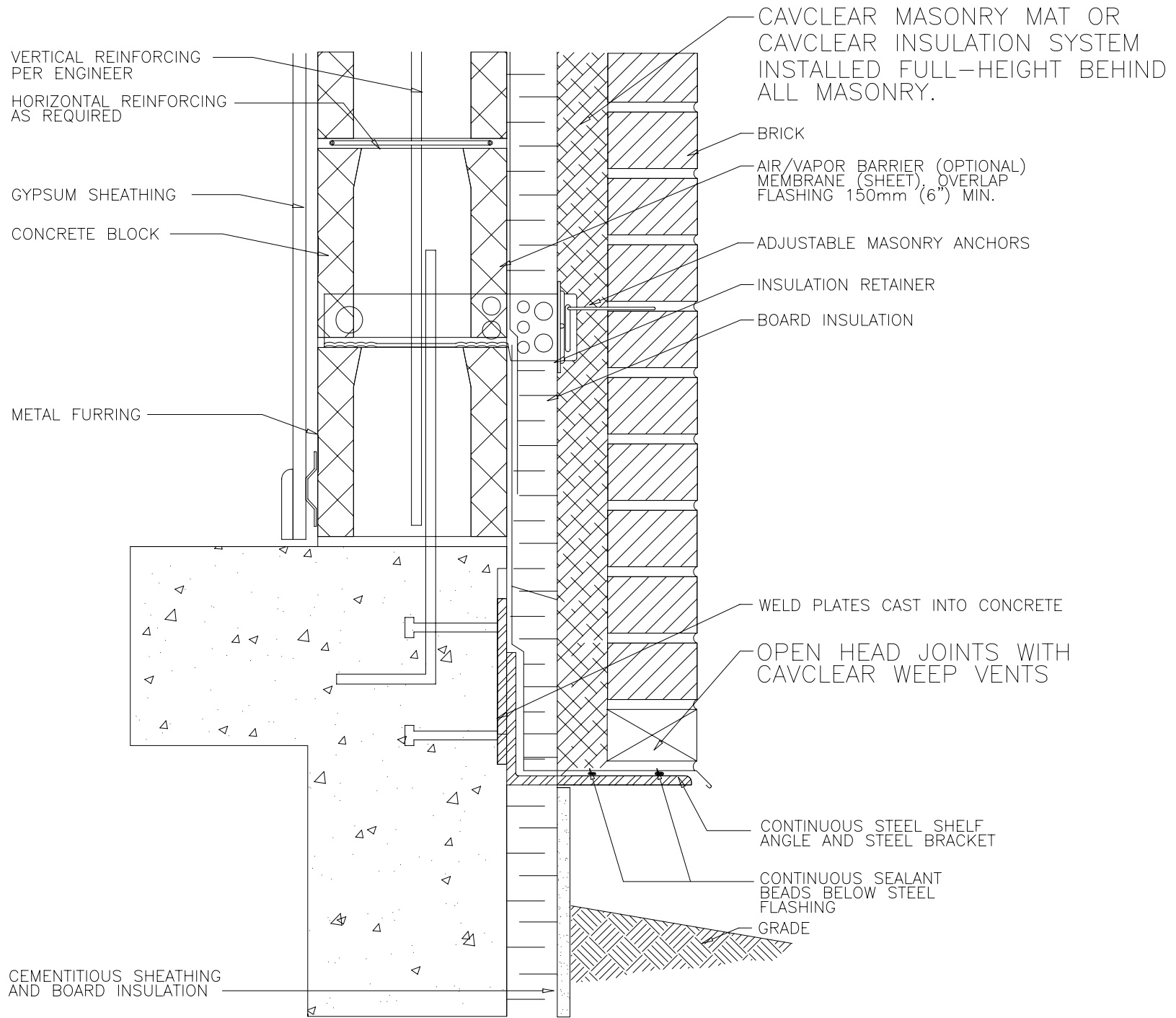
FOUNDATION WITH SHELF ANGLE DETAIL
